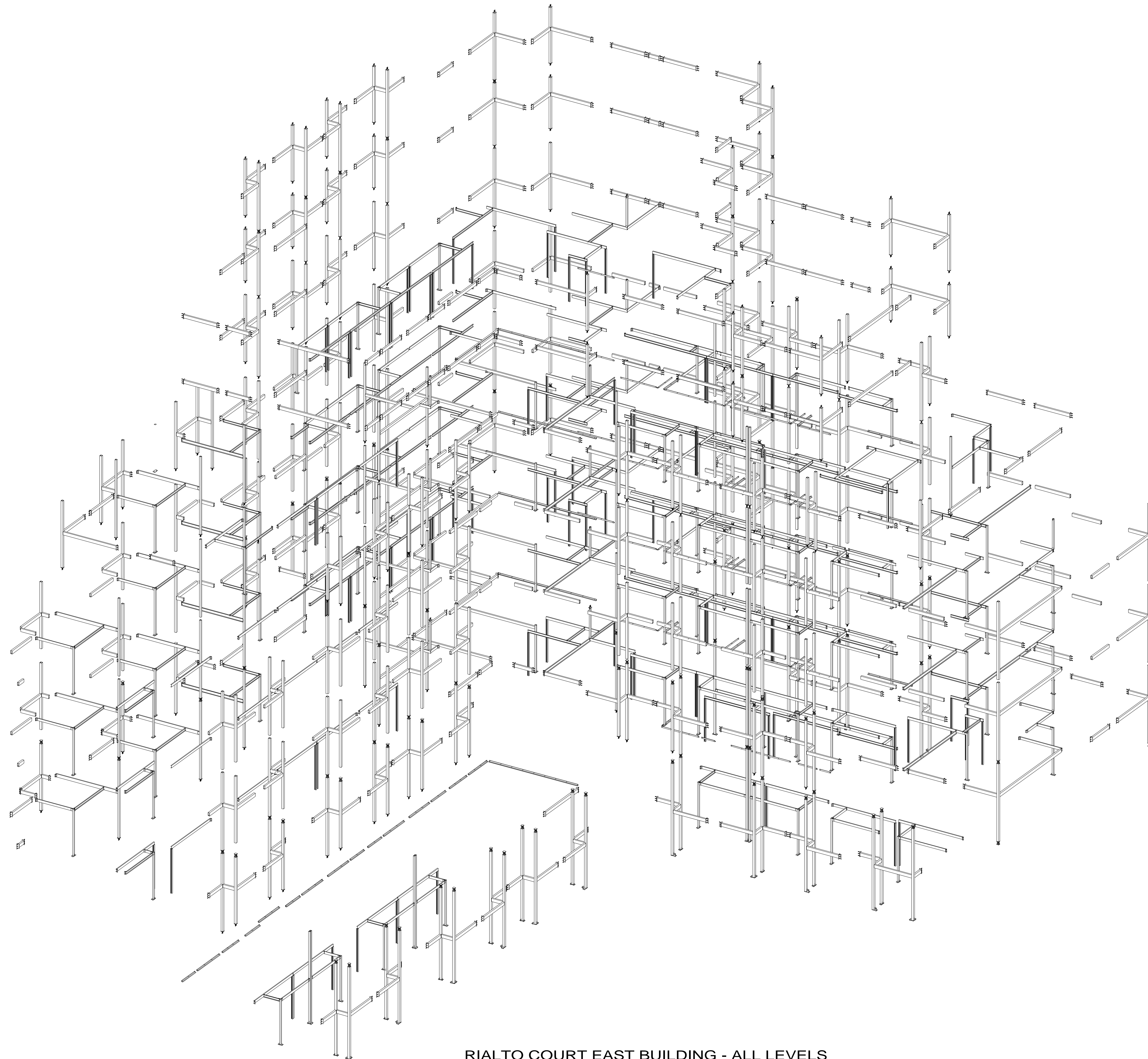
RIALTO COURT EAST BUILDING - ALL LEVELS (PERSPECTIVE VIEW)
